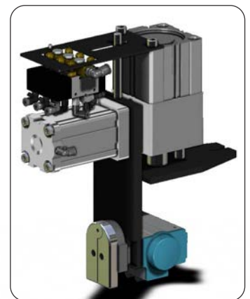
Brand new STITCH DOWN DEVICE (On demand).
